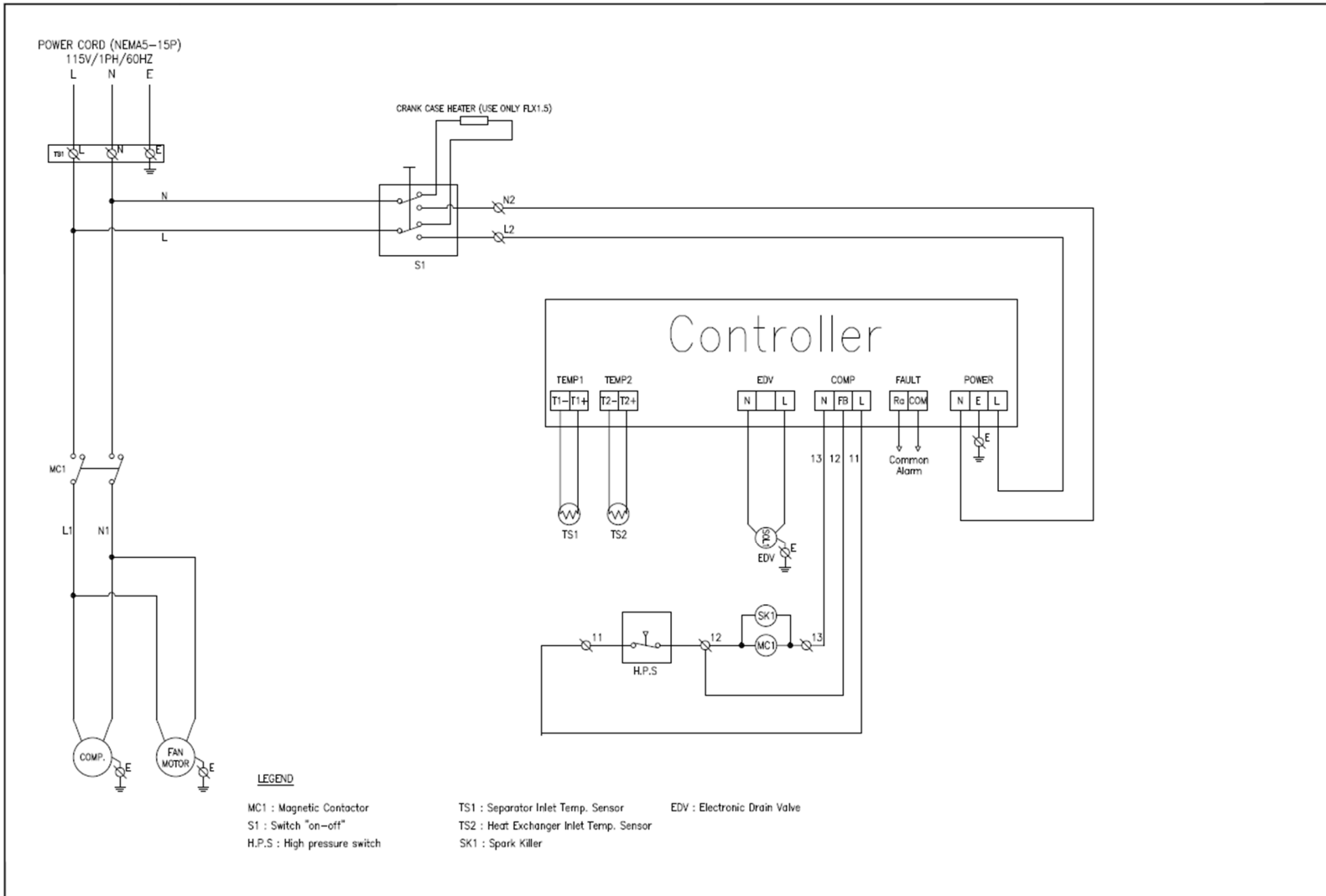
Figure 9A Models: DFXA 1.1~1.5(115V/1PH/60Hz)
