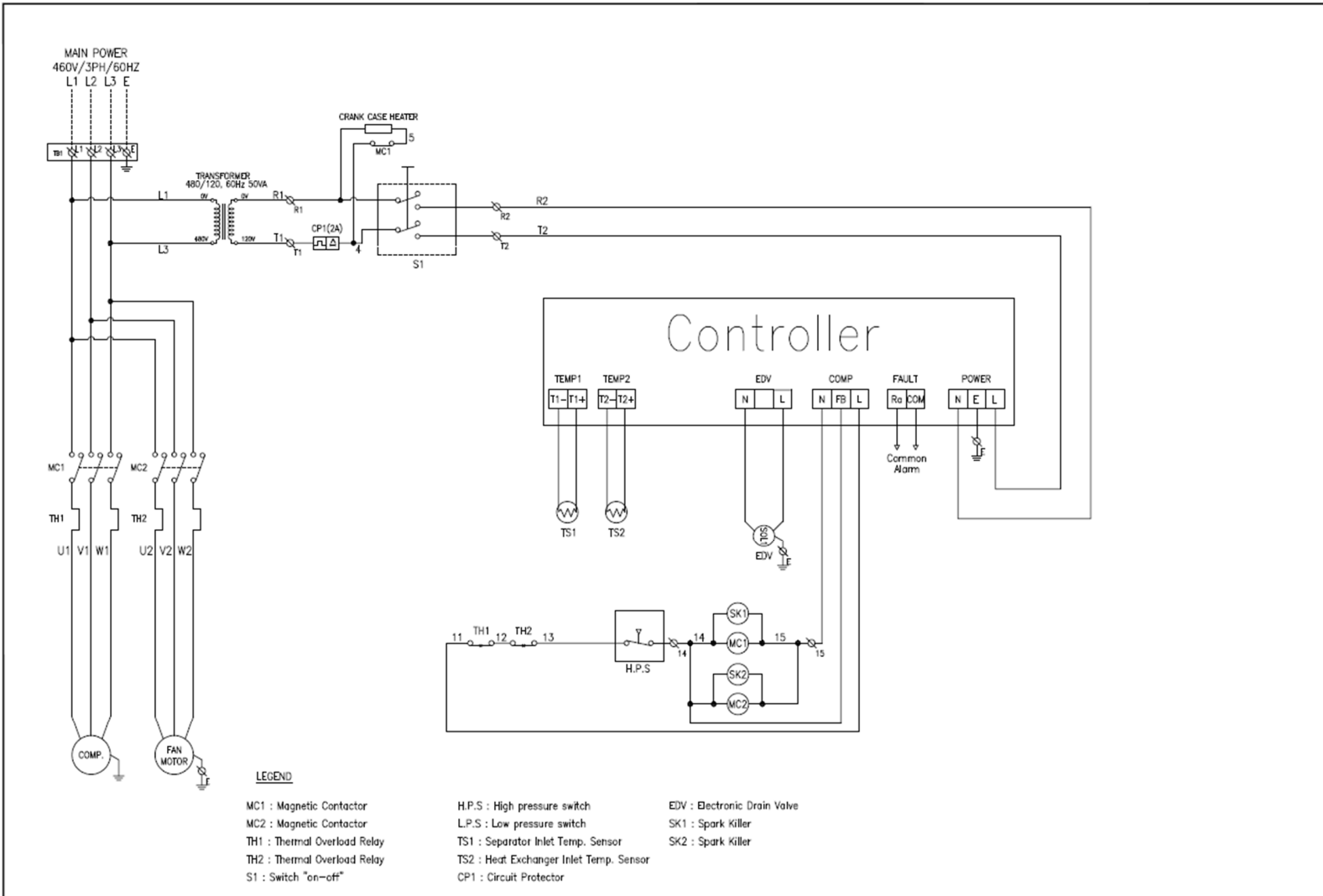
Figure 9B Model: DFXA 2.1-A (460V/3Ph/60Hz)
