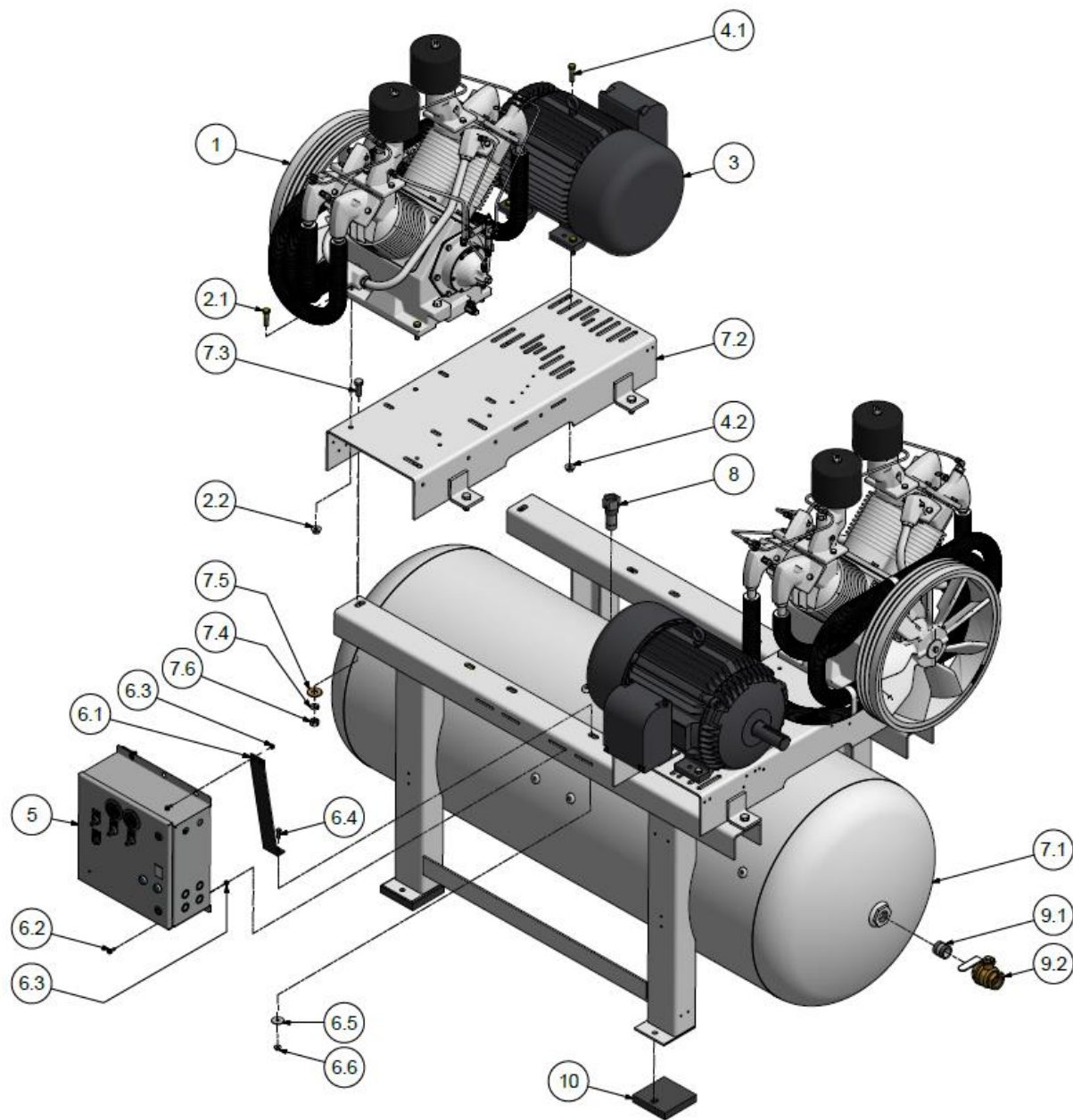
425CAD810-00 Ref Drawing
