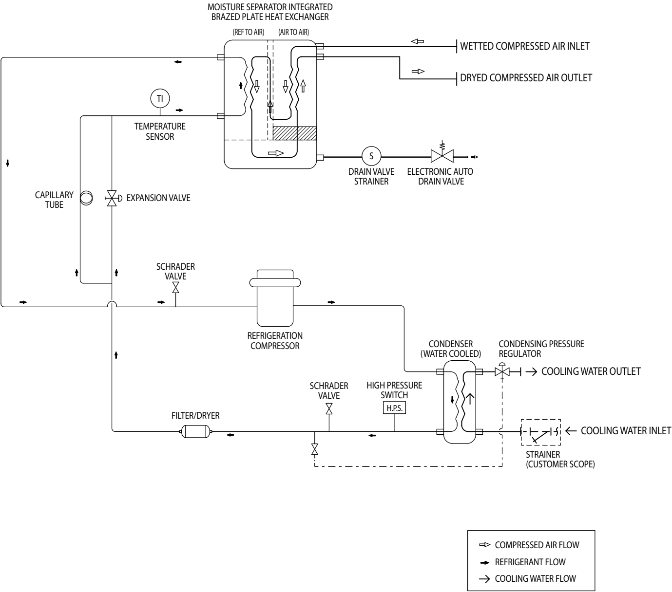
Air and Refrigerant Flow Schematic: Model HGEN600W
