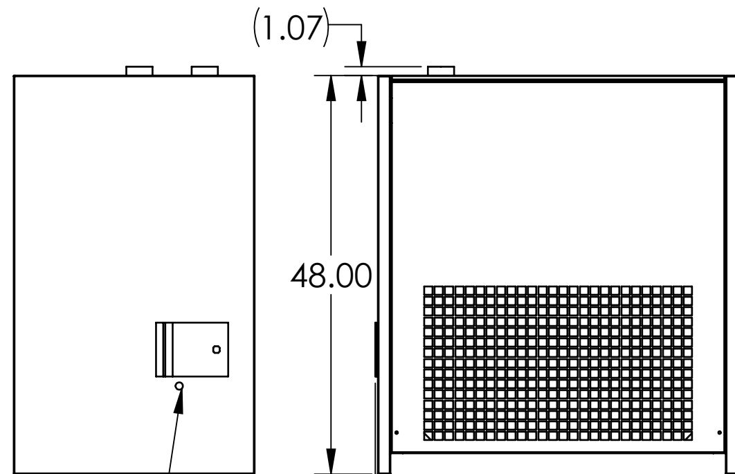
SIDE VIEW
