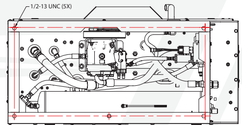
MOUNTING HOLES
